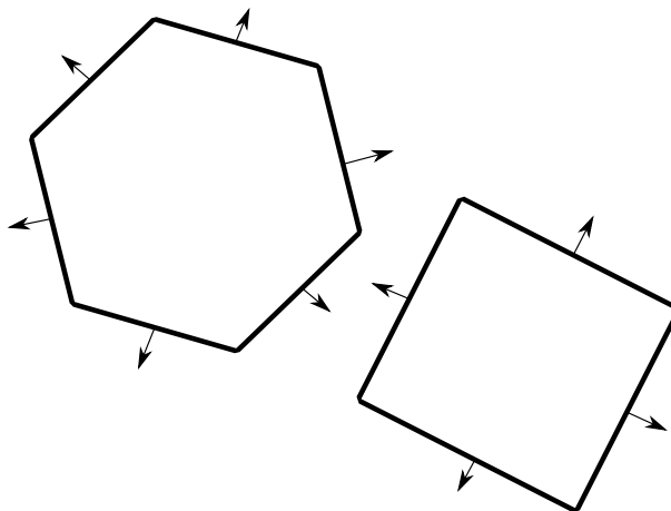
Figure 201: Finding the axes for the SAT (1/2)
